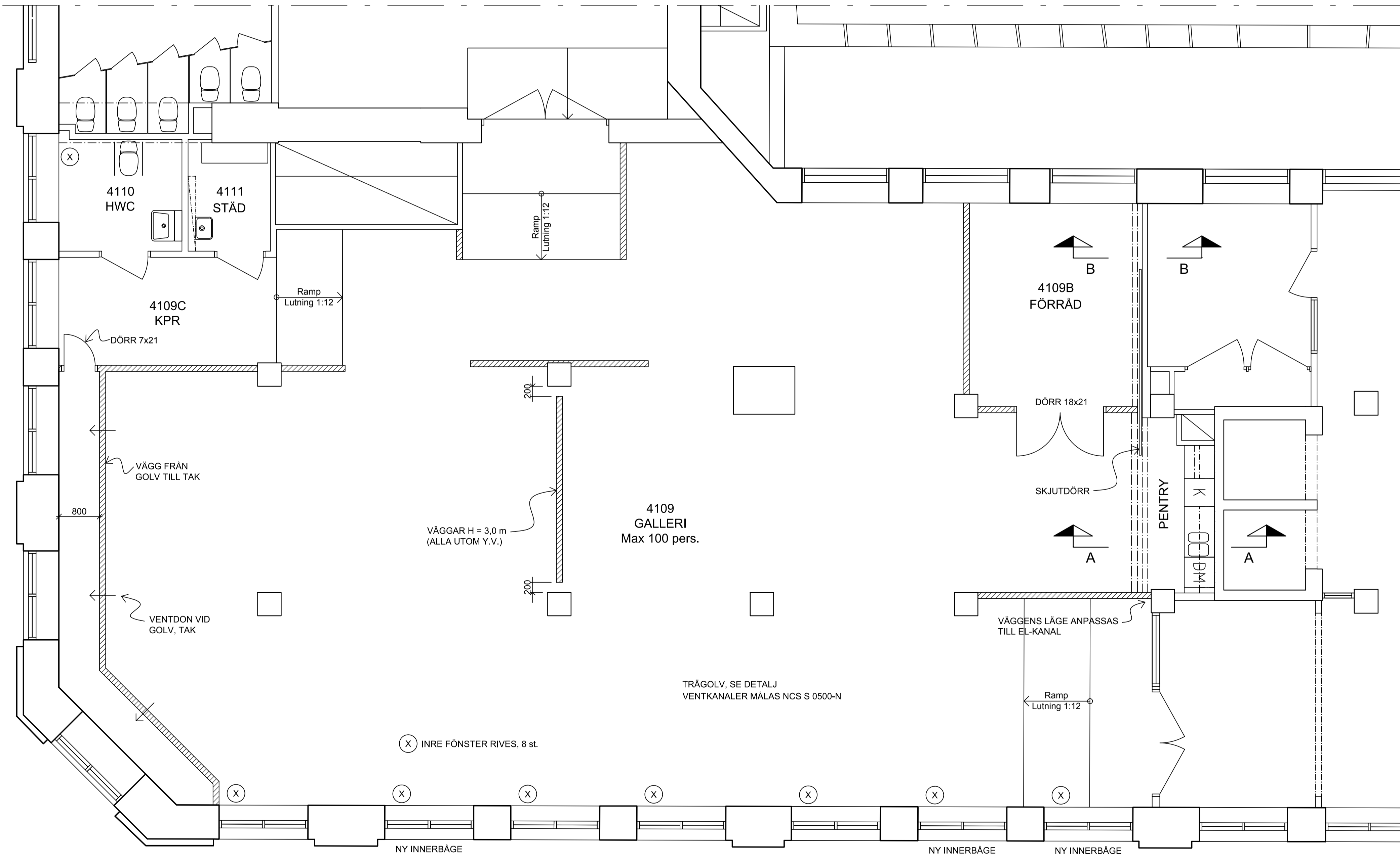
PLAN 1 Skala 1:50
